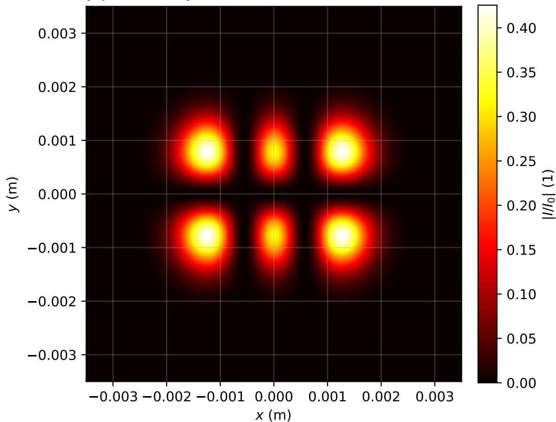
Intensity profile I(x, y, z = 2.468)/I_0 , P_{in}=0.5P_{cr} , artificial time
